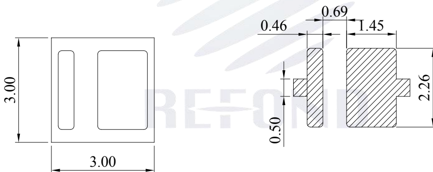
Fig.1-4 Bottom view
