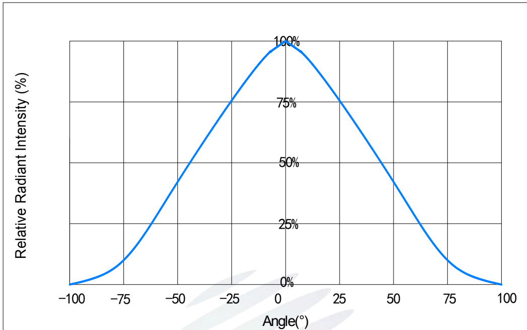
Fig 1-10 Radiation diagram
