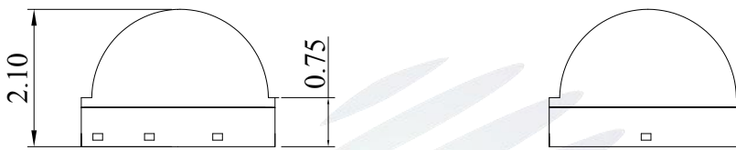
Fig.1-3 Side view
