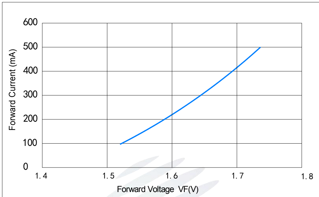
Fig 1-6 Forward Voltage Vs. Forward Current
