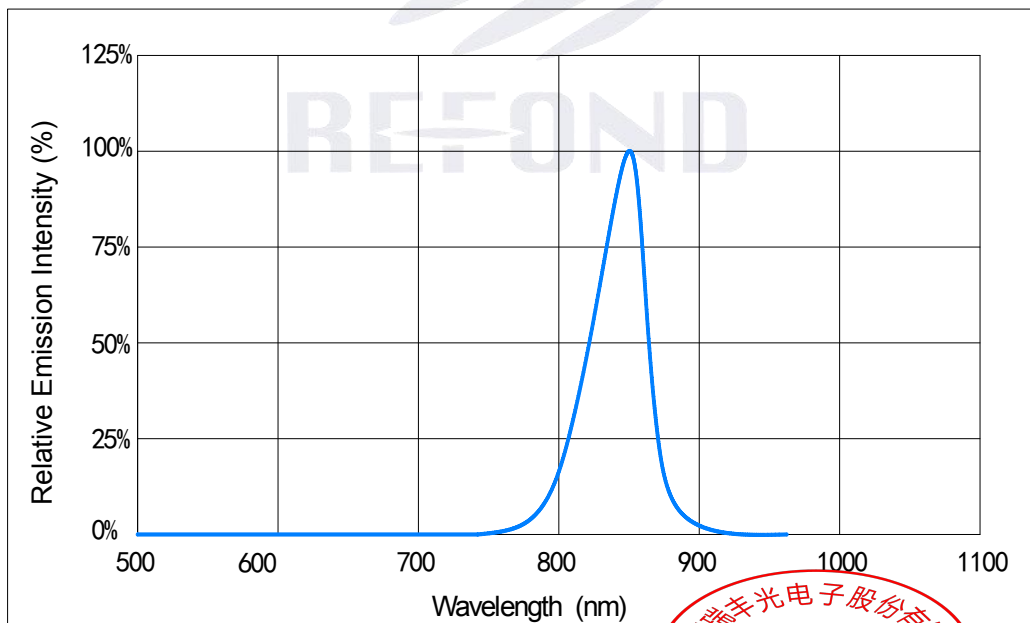
Fig 1-9 Spectrum Distribution
