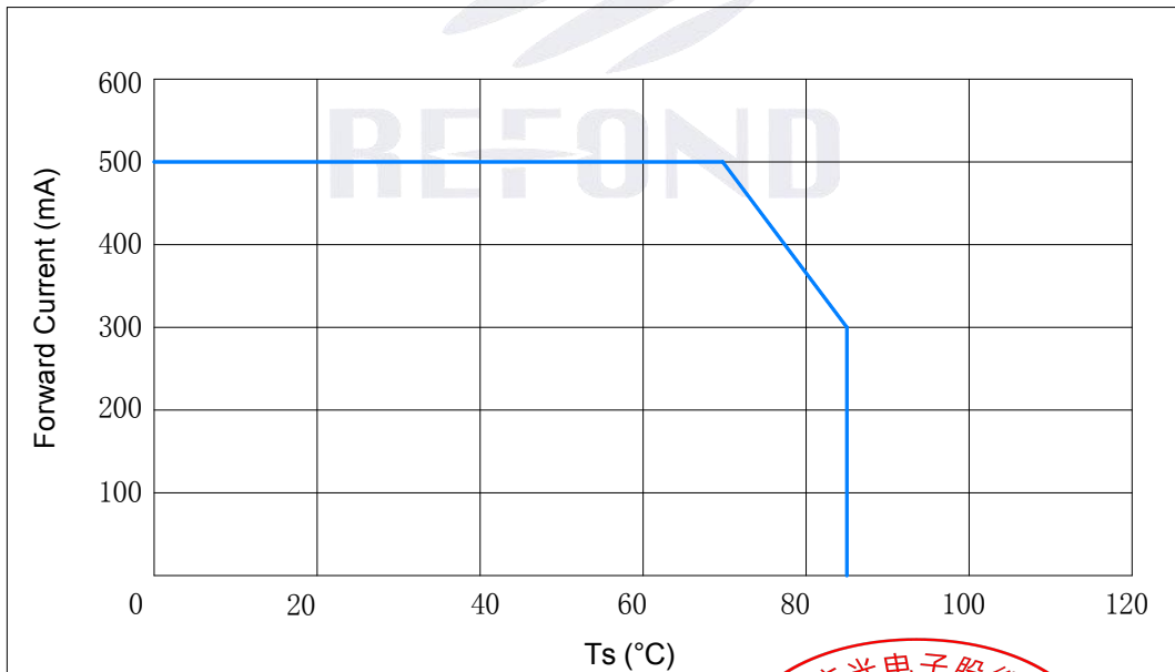
Fig 1-11 Ts Temperature Vs Forward Current
