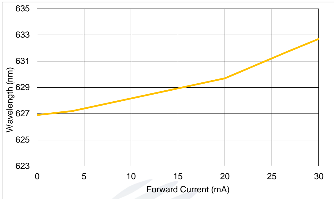
Fig.1-10 Forward Current Vs Dominant Wavelength (Ta=25°C) 正向电流与主波长关系曲线 (橙光)
