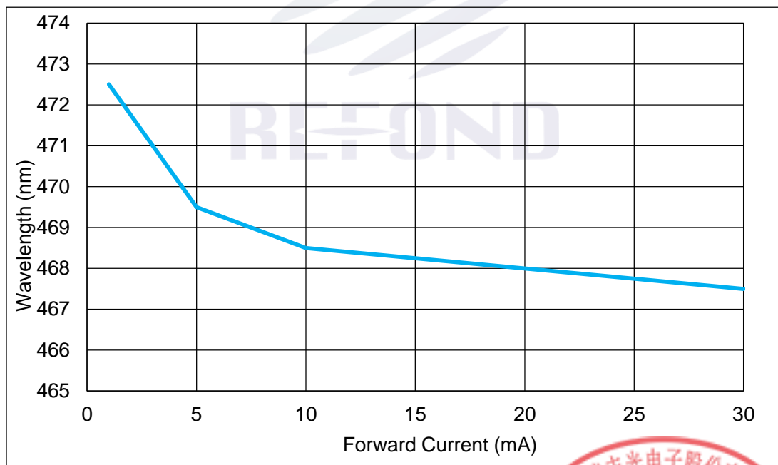
Fig.1-11 Forward Current Vs Dominant Wavelength (Ta=25°C) 正向电流与主波长关系曲线 (蓝光)
