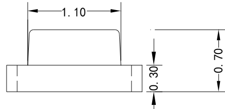
Fig.1-2 Side view 侧面视图
