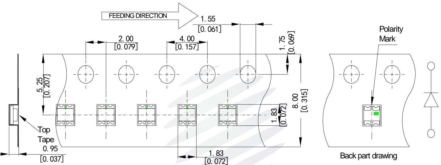
Fig.2-1 Carrier Tape Dimension 载带尺寸
