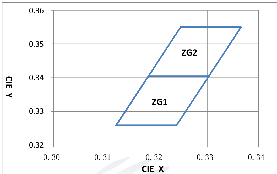
Fig. 1-6 The C.I.E Chromaticity Diagram CIE色度图
