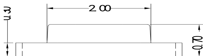
Fig.1-2 Side view 侧面视图
