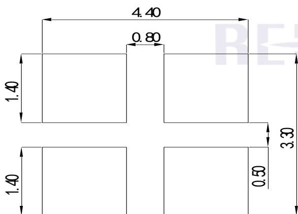
Fig.1-5 Soldering patterns 推荐焊盘
