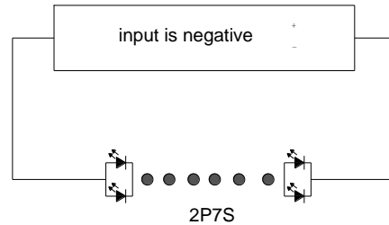
Fig.2-2 Product connection 产品电性图
