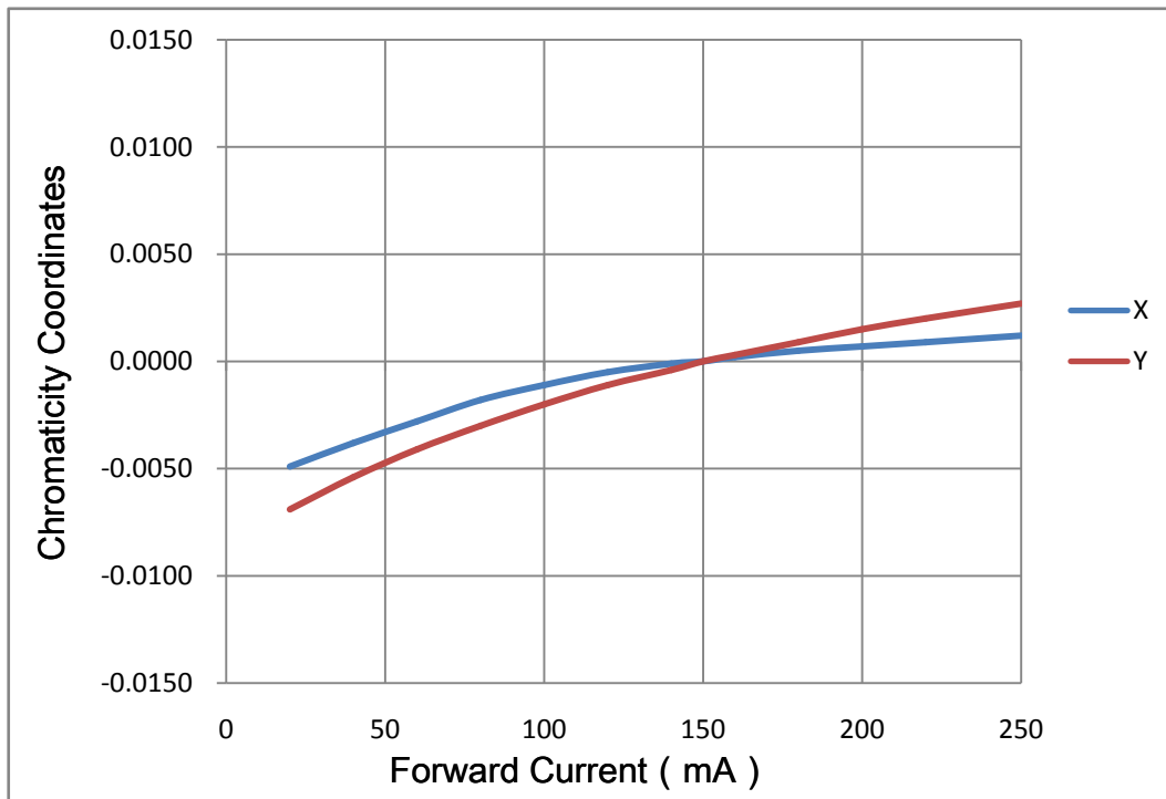
Fig. 1-13 Chromaticity Coordinate Vs Forward Current色坐标与正向电流特性曲线
