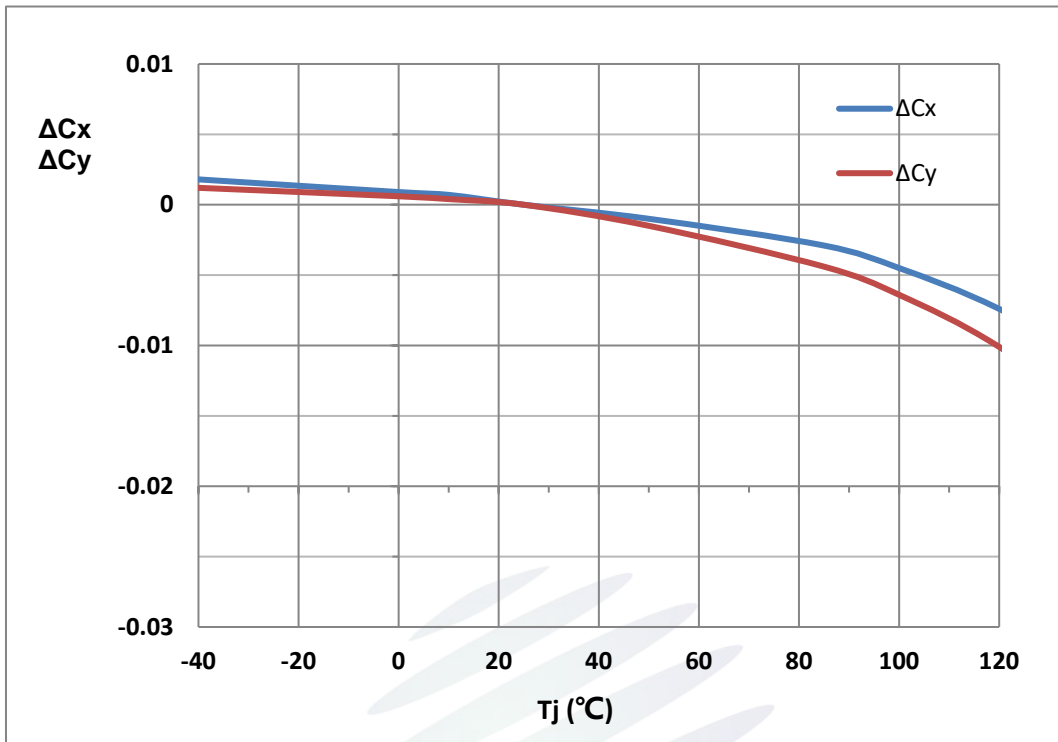
Fig. 1-13 Color coordinate shift Vs Junction Temperature 色坐标偏移与结温特性曲线
