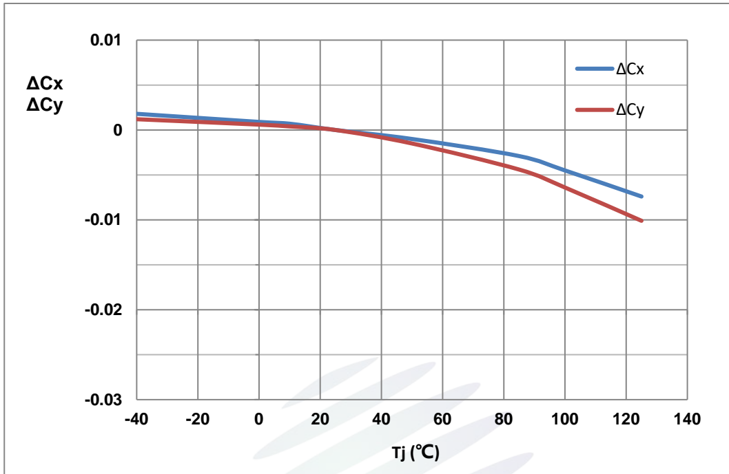
Fig. 1-13 Color coordinate shiftVs Junction Temperature色坐标偏移与结温特性曲线
