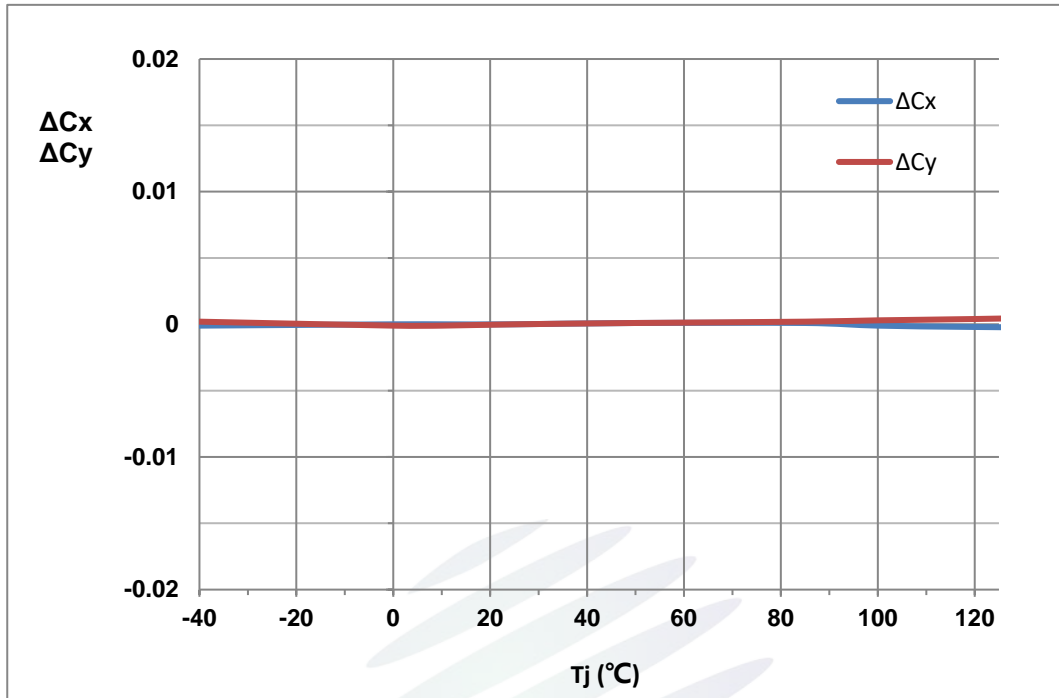
Fig. 1-13 Color coordinate shift Vs Junction Temperature 色坐标偏移与结温特性曲线
