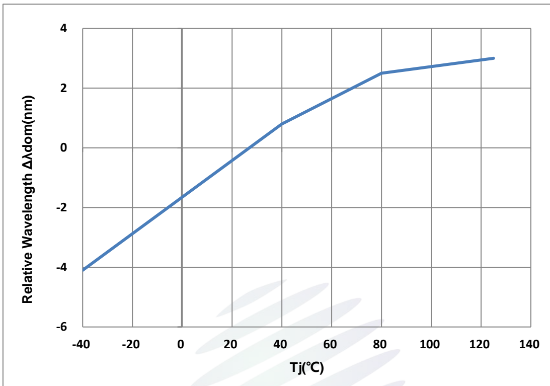
Fig. 1-13 Wavelength Coordinate Shift Vs Junction Temperature 色坐标偏移与结温特性曲线
