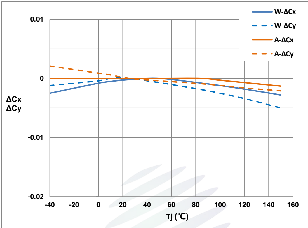
Fig. 1-14 Chromaticity Coordinate Shift Vs Junction Temperature 色坐标偏移与结温特性曲线
