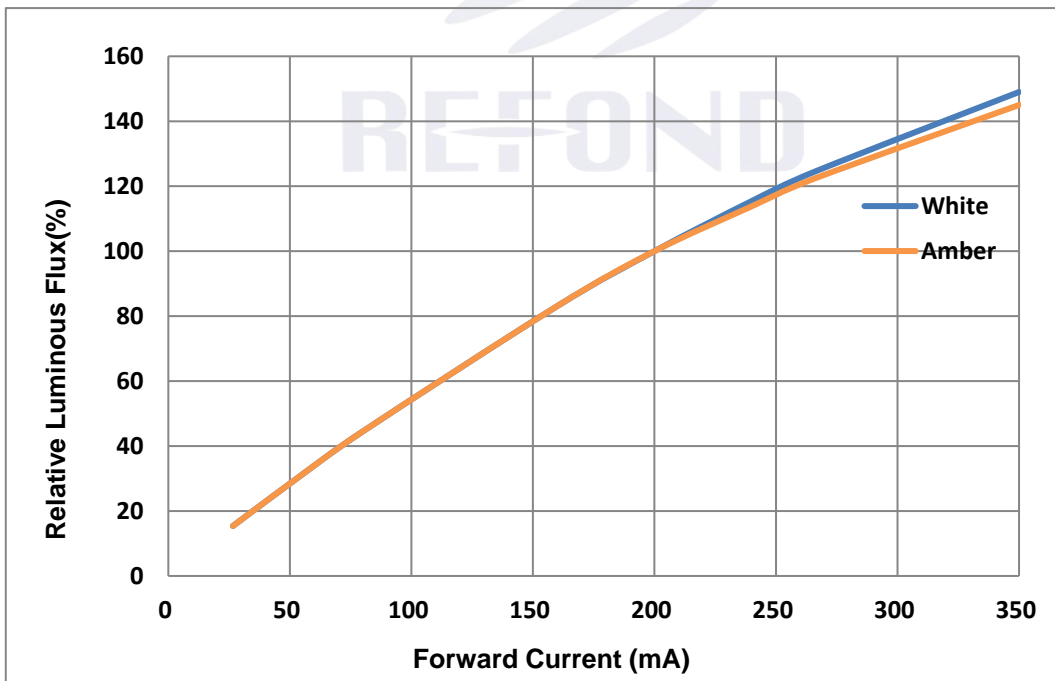
Fig. 1-9 Forward Current Vs Relative Intensity 正向电流与相对光强特性曲线
